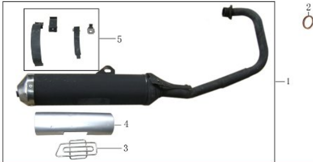
F-14 排气消声器总成 EXHAUST MUFFLER
