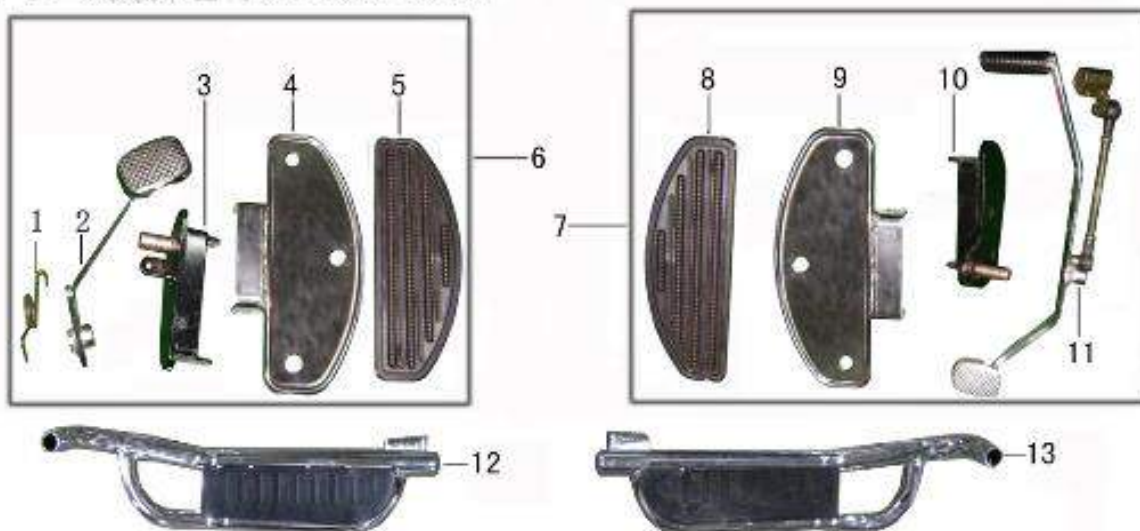
F-14 搁脚组合 FOOTREST ASSY
